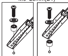
M5×25mm(C1) M6×25mm(B1)
